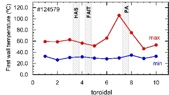
First wall
