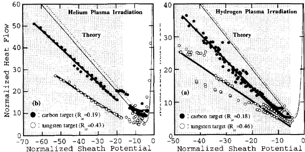
Fig. 6. The normalized plasma heat flows from experiment and theory. Thin solid curves are obtained from Eq. (3), simple sheath theory, that does not include the effects of ion reflection and surface recombination. Dashed lines come from Eq. (5) with R_{ie} = 0 and typical electron temperatures T_e = 15 eV for hydrogen plasma and 10 eV for helium plasma are substituted, respectively. The hatched regions are the ion saturation region, in which ion contribution to the heat flow dominate. The experimental data points are fitted by the bold solid lines. (a) Hydrogen plasma \rightarrow carbon or tungsten, (b) helium plasma \rightarrow carbon or tungsten.
