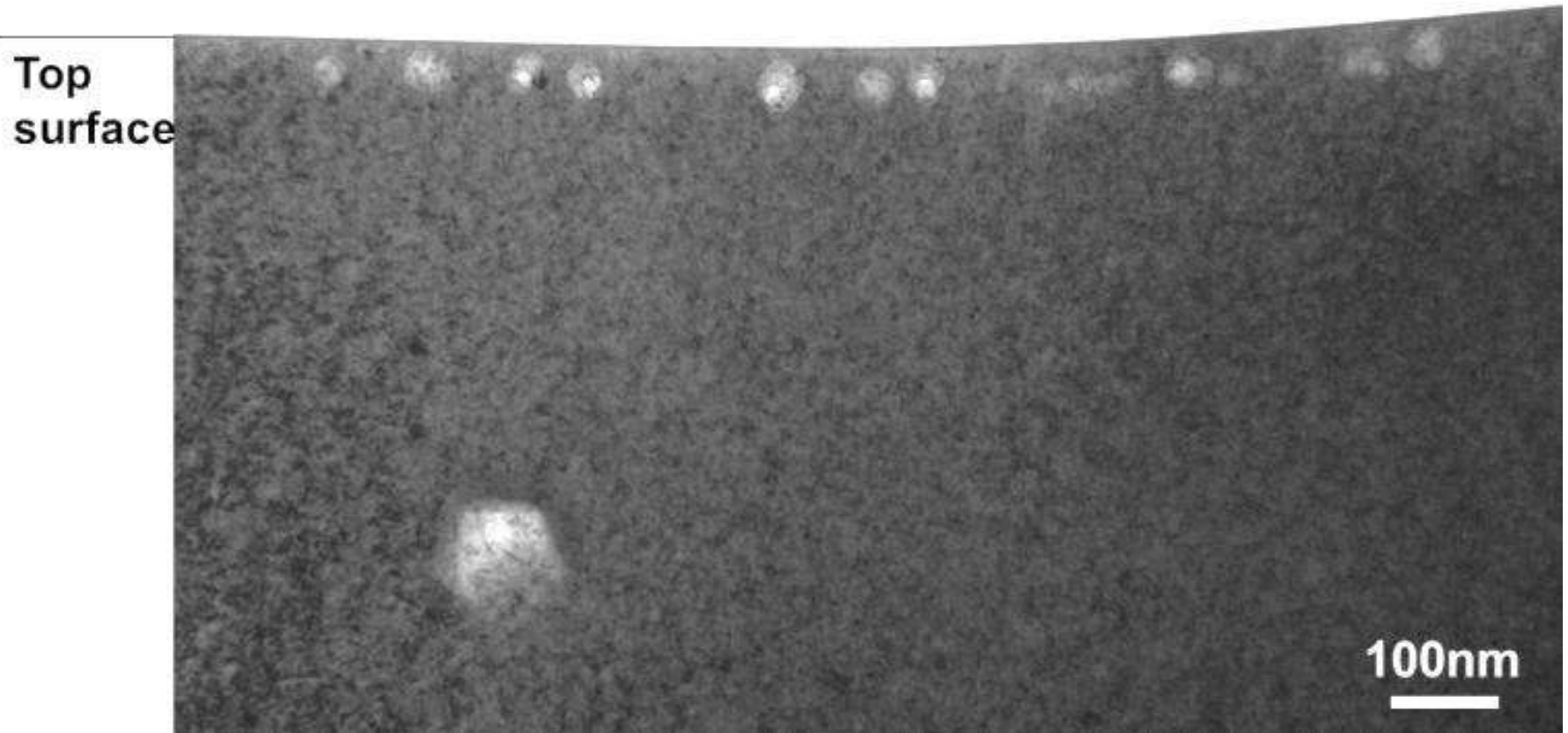
TEM images of W irradiated with LHD divertor plasmas. 100-200eV, \sim 10^{22-23} ions/m 2 s.
