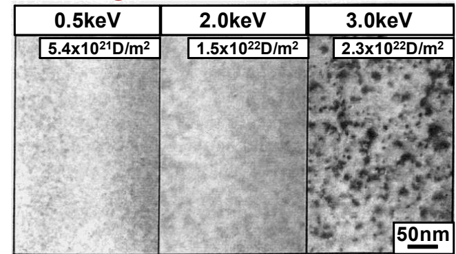
TEM images of W irradiated with various energy of D + in room temperature.
