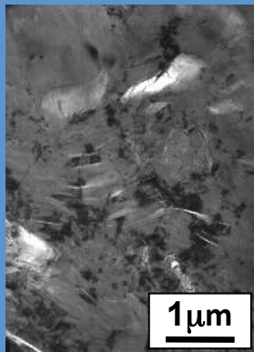
TEM image of virgin IG-430U and corresponding diffraction pattern.
