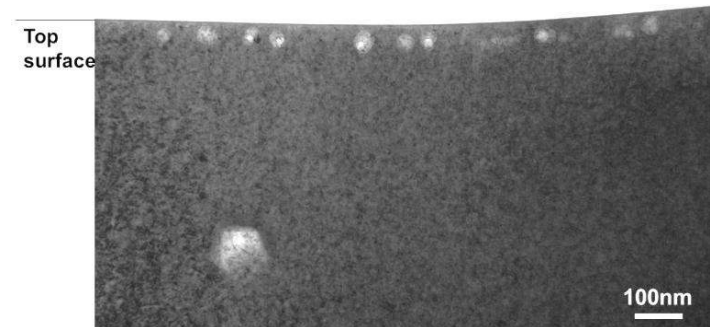
TEM images of W irradiated with LHD divertor plasmas. 100-200eV, \sim 10^{22-23} ions/m 2 s.
