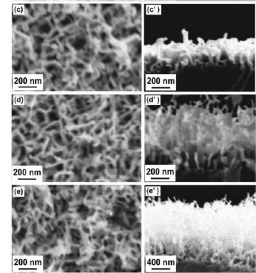
Fig. 1. Growth process of W-fuzz irradiated with low energy He ion (up to 5.5 \times 10^{25} \text{He/m}^2 ) [1].
