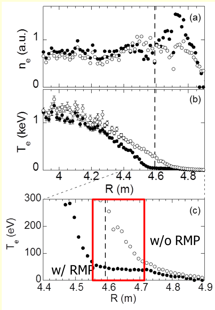
Radial profiles of n_e and T_e
