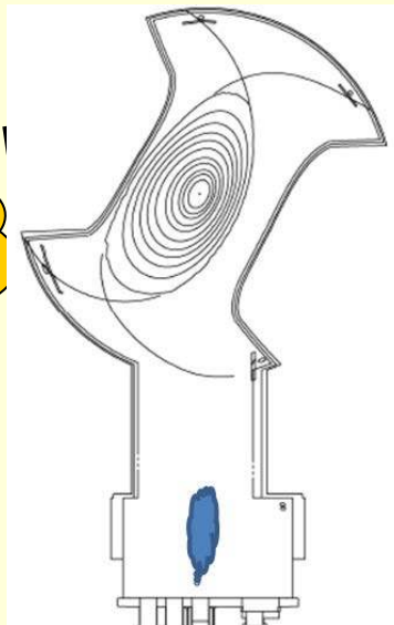
Gas puffing from a bottom port
